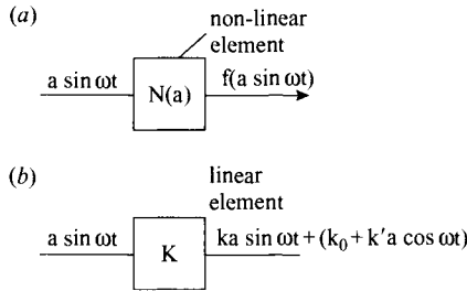
Figure 13.4 a A non-linear element b A linear approximation to the non-linear element in (a)
