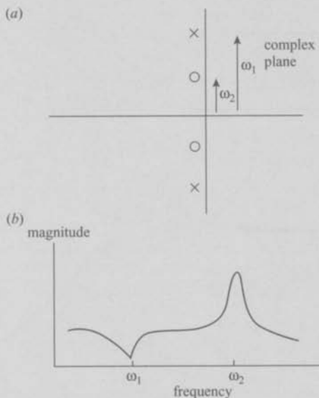
Figure 5.9 a A pole-zero diagram in which the poles and zeros are close to the imaginary axis b The form of the (magnitude) frequency response corresponding with (a)
